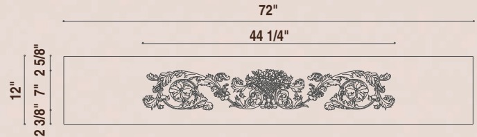
RH6082 ~ Rinceau Scrolls with Floral Basket Range Hood 72" x 12" x 1 1/4"
