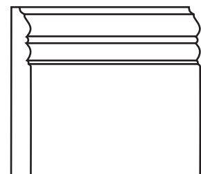
BA499 Base 5/8" x 5 1/4" 15.9 x 133.4 mm
