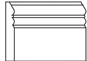
BA498 Base 5/8" x 4 1/4" 15.9 x 108 mm
