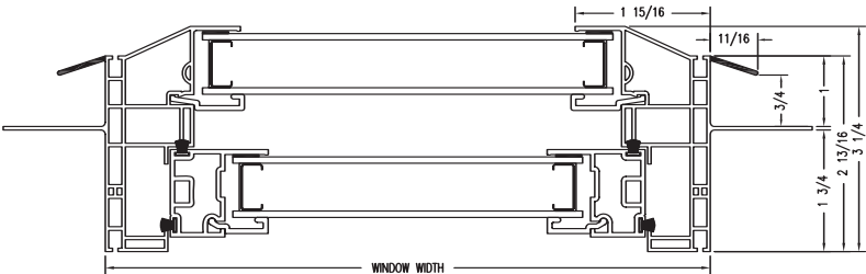
3500 SINGLE HUNG WITH J-CHANNEL HORIZONTAL CROSS SECTION
