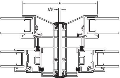
3500 SINGLE HUNG HORIZONTAL MULL CROSS SECTION
