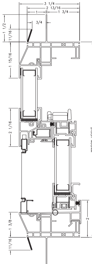
3500 SINGLE HUNG WITH J-CHANNEL VERTICAL CROSS SECTION
