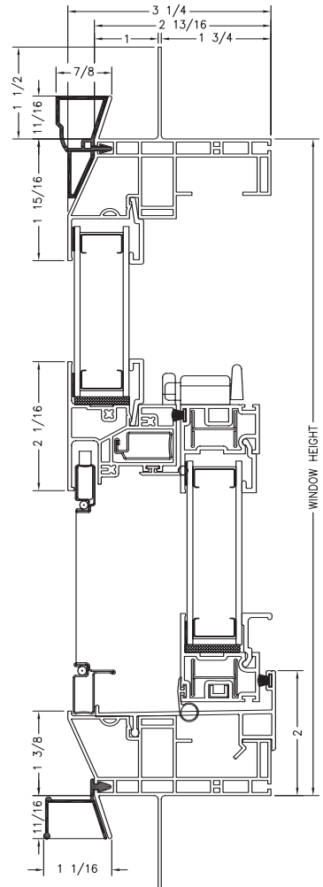
3500 SINGLE HUNG WITH OPTIONAL BRICKMOLD VERTICAL CROSS SECTION
