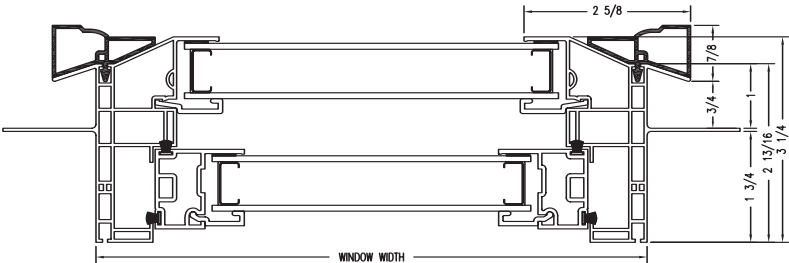
3500 SINGLE HUNG WITH BRICKMOULD HORIZONTAL CROSS SECTION
