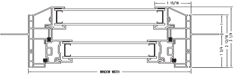
3500 SINGLE HUNG HORIZONTAL CROSS SECTION
