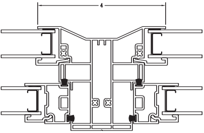
3500 SINGLE HUNG INTERMEDIATE JAMB HORIZONTAL CROSS SECTION
