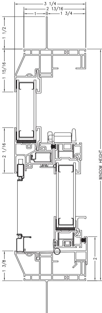
3500 SINGLE HUNG VERTICAL CROSS SECTION
