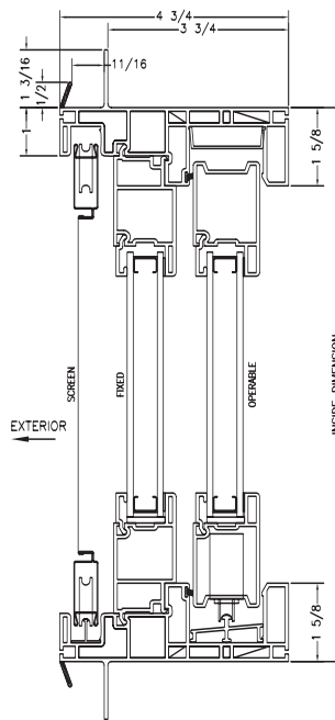
VERTICAL DETAIL WITH J-CHANNEL
