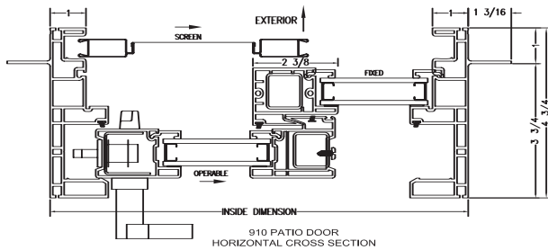
HORIZONTAL DETAIL
