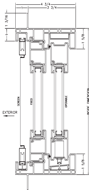
VERTICAL DETAIL
