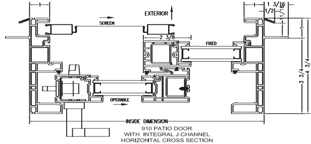
HORIZONTAL DETAIL WITH J-CHANNEL
