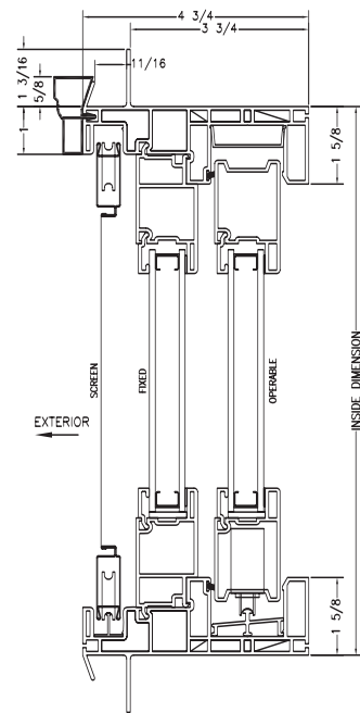
VERTICAL DETAIL WITH BRICKMOULD
