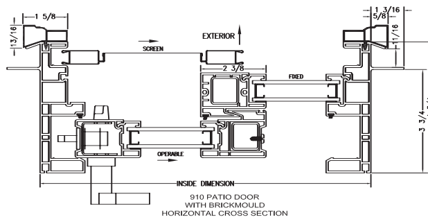
HORIZONTAL DETAIL WITH BRICKMOULD
