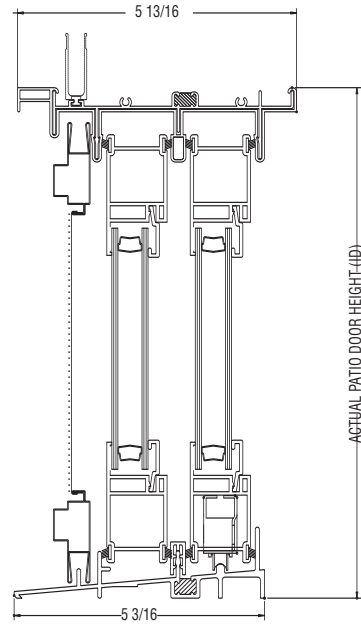
6" FRAME VERTICAL DETAIL
