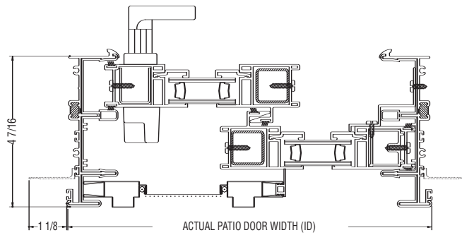
4" FRAME HORIZONTAL DETAIL
