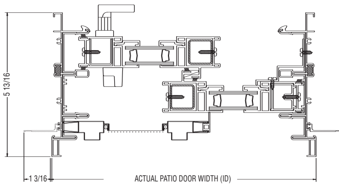
6" FRAME HORIZONTAL DETAIL
