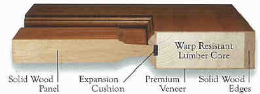
Charleston Section View with COVE & BEAD Profile
