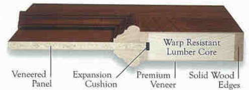
Brittany Section View
