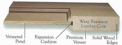
Newport Section View with COVE & BEAD Profile
